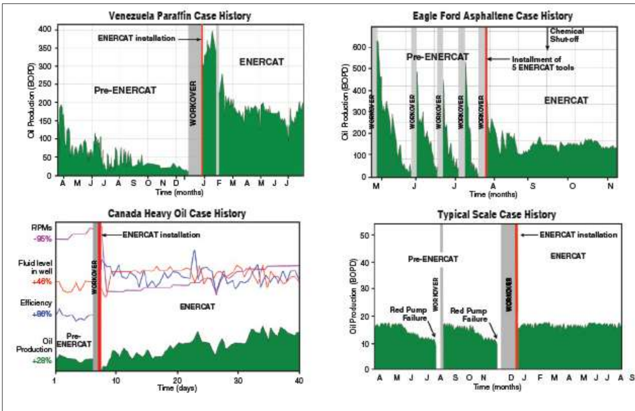
Paraffin, asphaltene, scale and heavy oil case history graphs show stabilization and increased production at the end of standard workovers after installing the Enercat™ downhole tool from Revelant Nanofluidity Technology.
