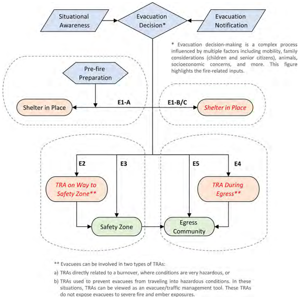
Fig. 5. Flow chart depicting generalized evacuation scenarios. Red text indicates hazard.
