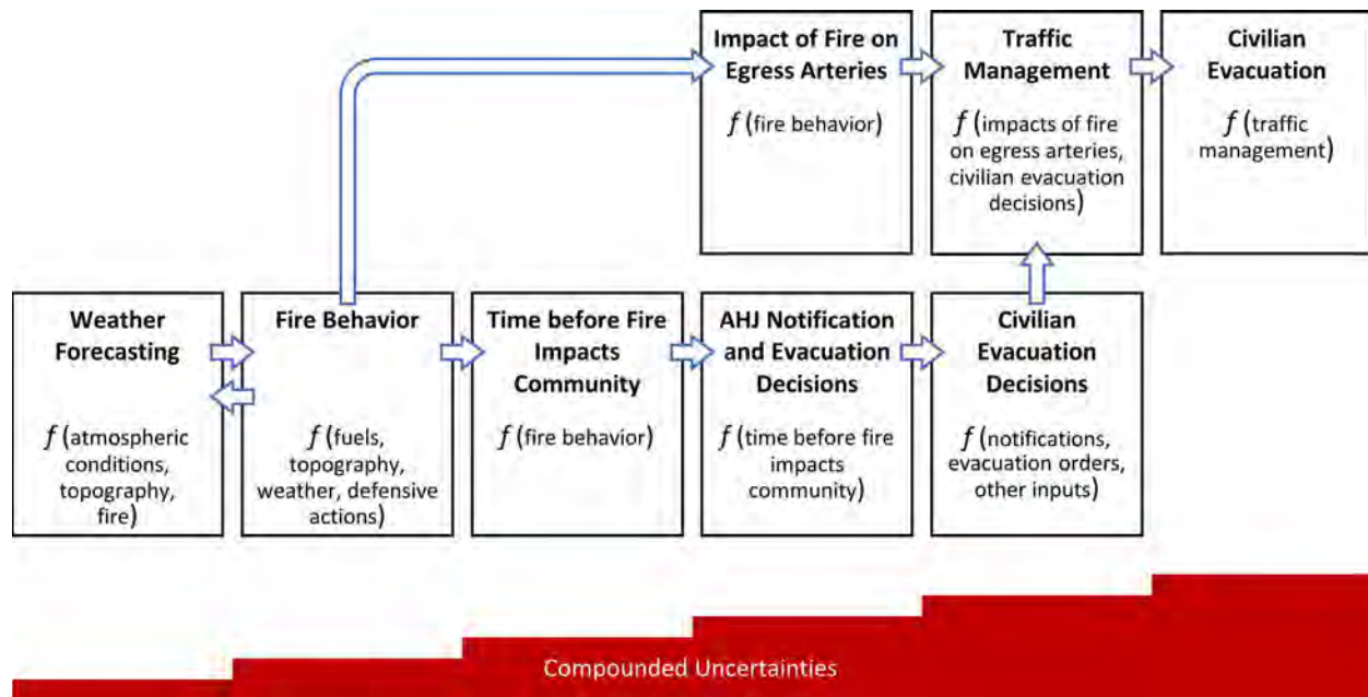
Fig. 3. Linked modules associated with evacuation predictions. Uncertainties are compounded and propagate from left to right and illustrated in red (not to scale).
