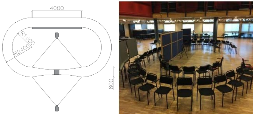
Figure 3 – a) Schematic view of the dimensions in millimetres of the circuit and the location of the camera. The third camera was filming from above. b) View of the circuit in the room
