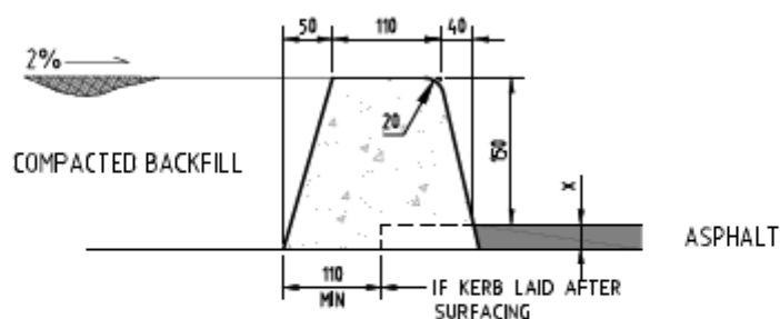
BARRIER KERB DETAIL - TYPE 2
