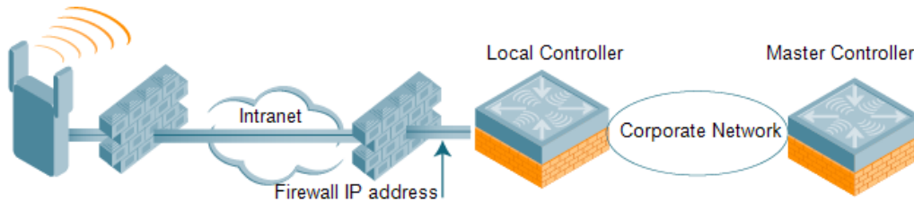
Figure 77 Remote AP in a Multi-Controller Environment
