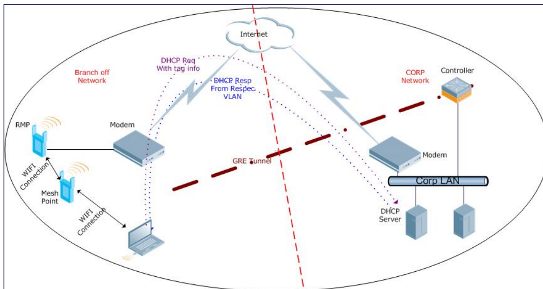
Figure 57 Working of RMP
