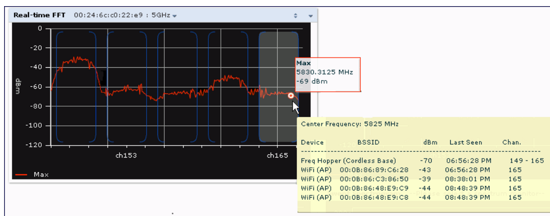
Figure 124 Real-Time FFT
