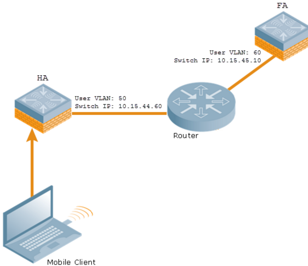
Figure 71 Sample IPv6 L3 Mobility Configuration
