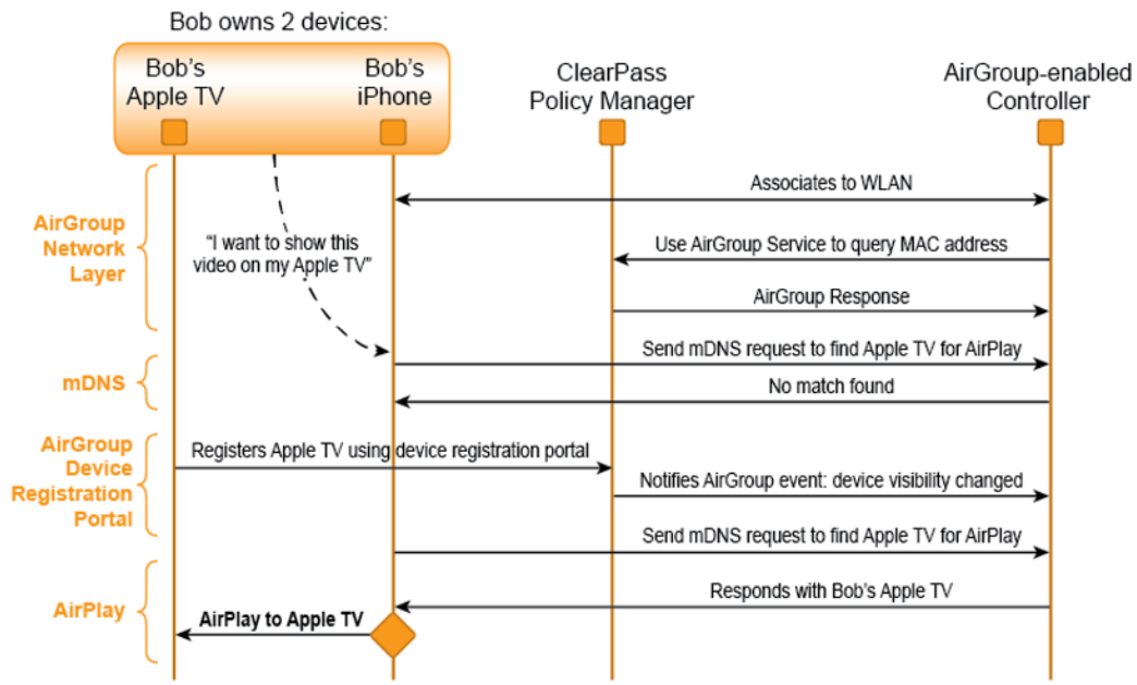
Figure 207 AirGroup Enables Personal Device Sharing
