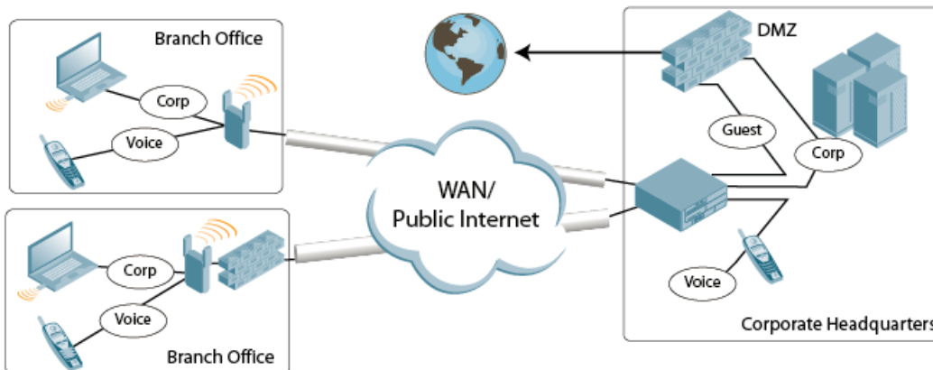
Figure 81 Remote AP with Single Controller
