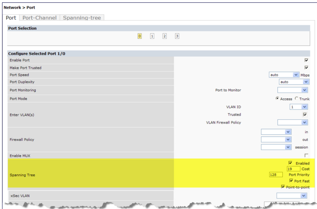
Figure 67 Configuring RSTP
