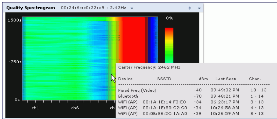
Figure 123 Quality Spectrogram
