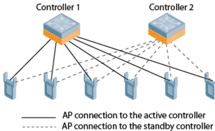
Figure 63 1:1 Active/Standby Deployment
