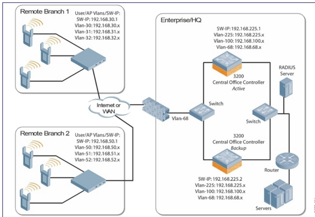
Figure 27 Sample OSPF Topology
