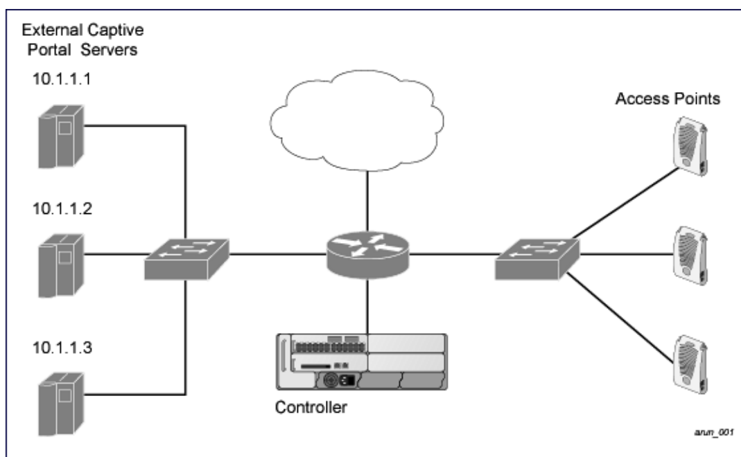
Figure 240 Example NAT-Mode Topology
