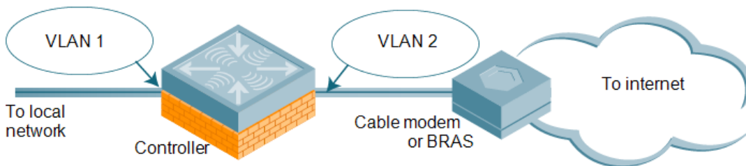
Figure 17 IP Address Assignment to VLAN via DHCP or PPPoE
