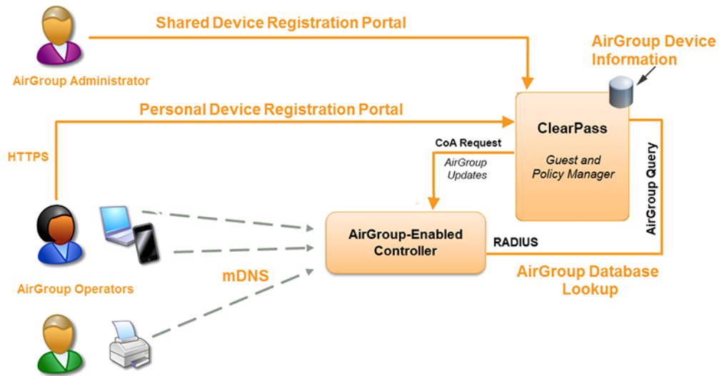
Figure 208 AirGroup in a Typical Wireless Deployment
