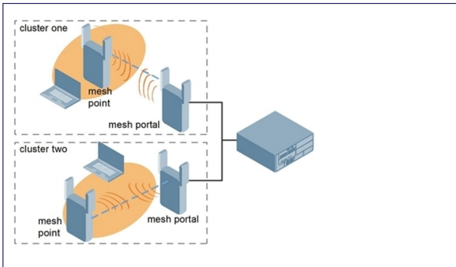
Figure 56 Sample Mesh Clusters
