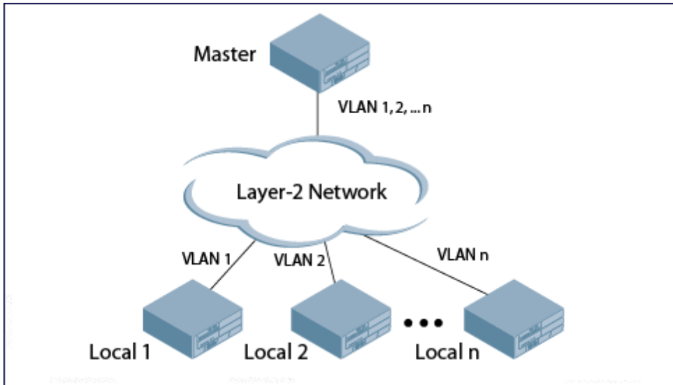
Figure 66 Redundant Topology: Master-Local Redundancy
