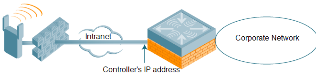
Figure 75 Remote AP with Controller on Public Network
