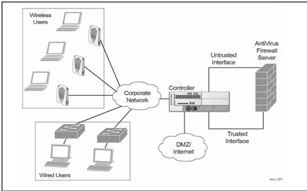
Figure 235 ESI-Fortinet Topology
