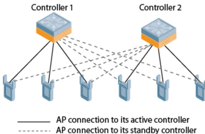
Figure 62 Active-Active HA Deployment
