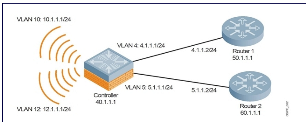
Figure 22 WLAN OSPF Topology
