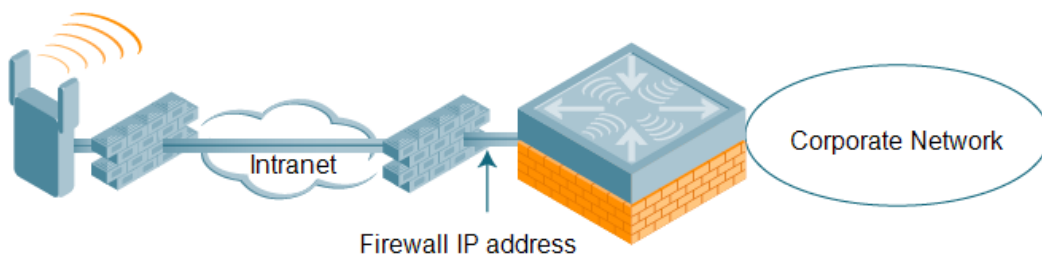
Figure 76 Remote AP with Controller Behind Firewall
