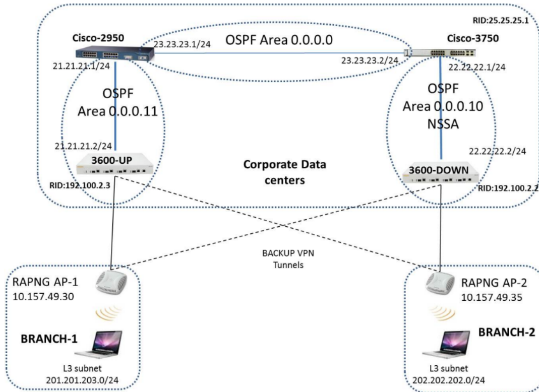
Figure 28 Controller Not-So-Stubby-Area (NSSA) and Normal Area
