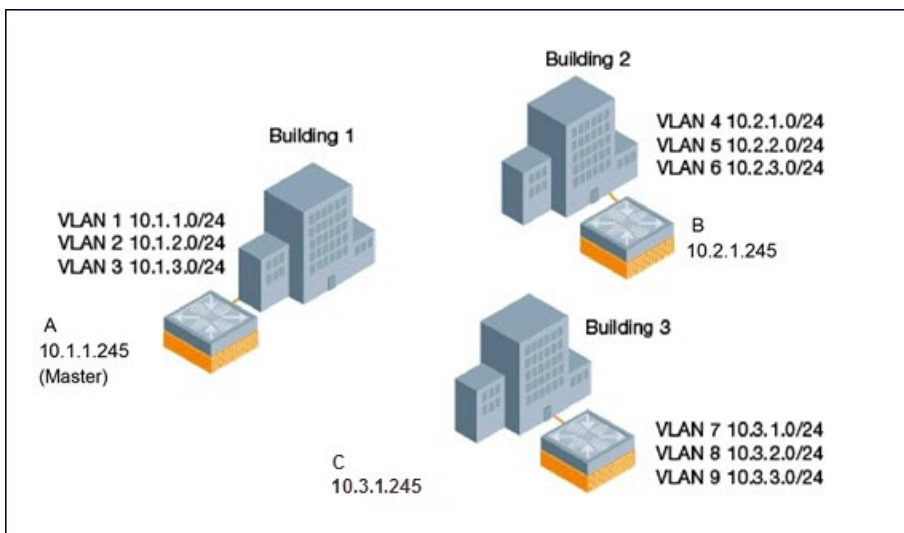
Figure 70 Example Configuration: Campus-Wide
