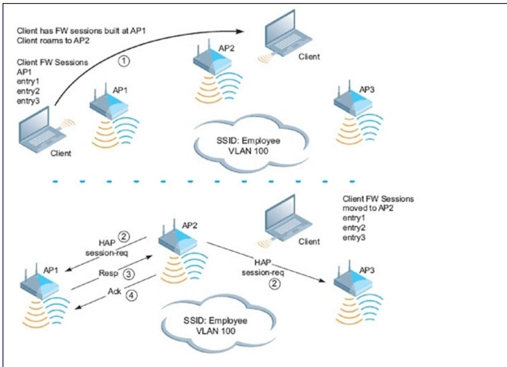
Figure 72 Bridge Mode Mobility
