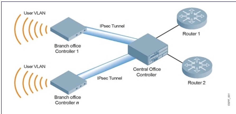
Figure 23 Branch Office OSPF Topology
