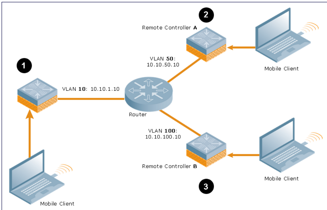
Figure 73 Inter-controller Mobility
