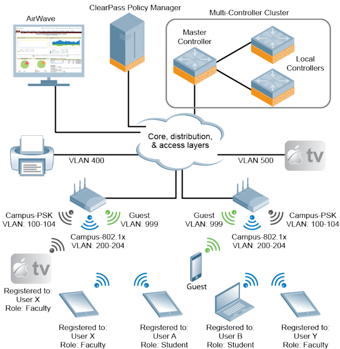
Figure 209 Integrated AirGroup Network Topology
