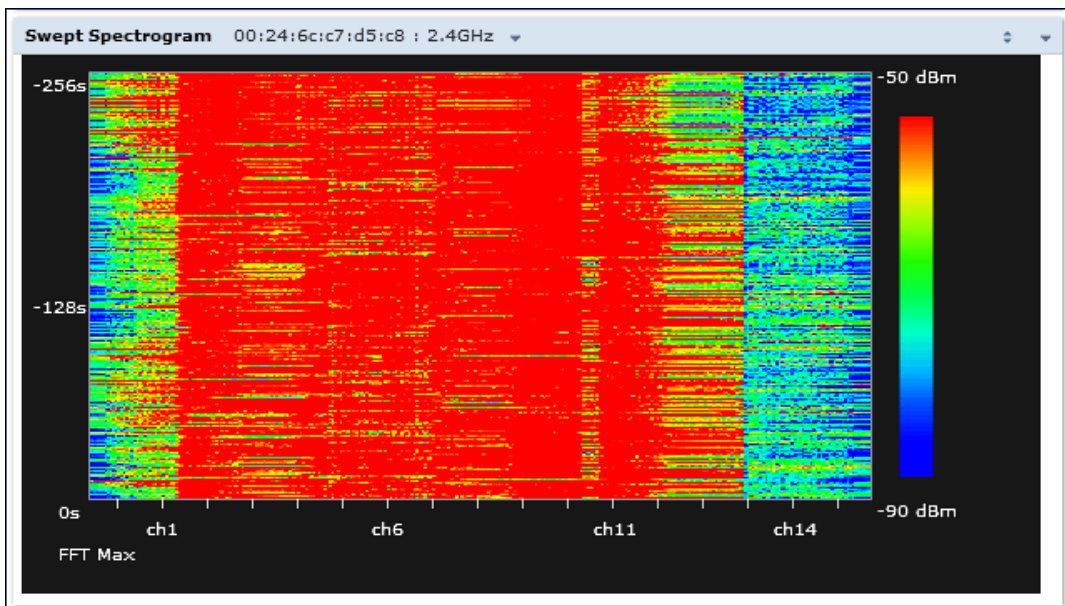
Figure 128 Swept Spectrogram
