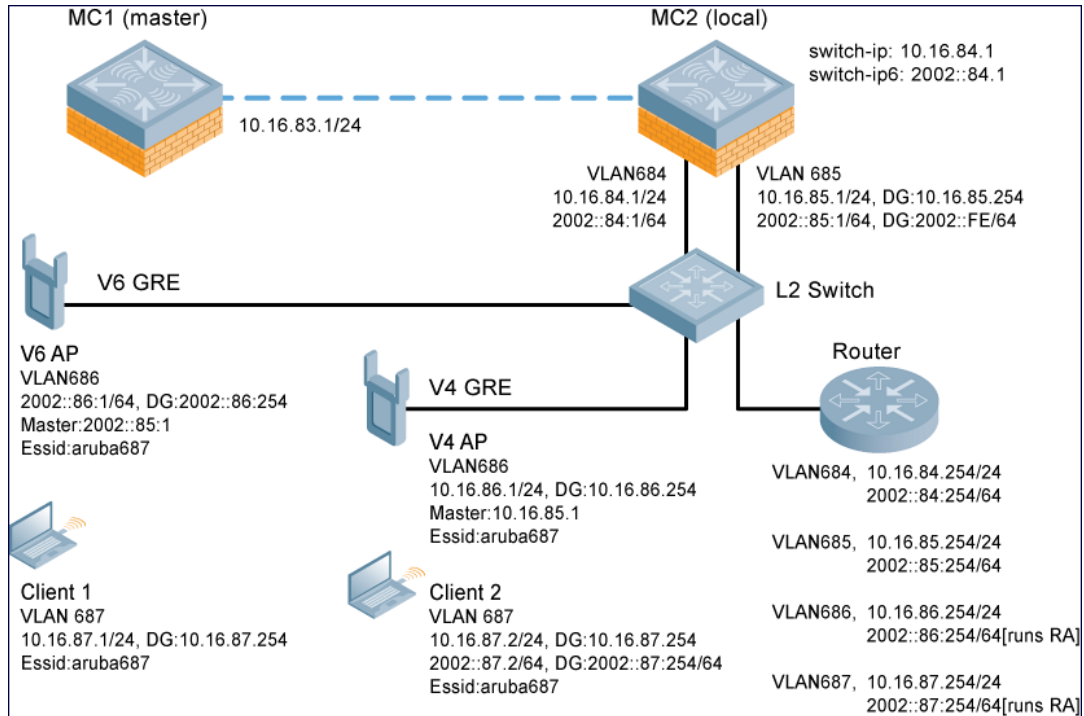
Figure 21 IPv6 Topology
