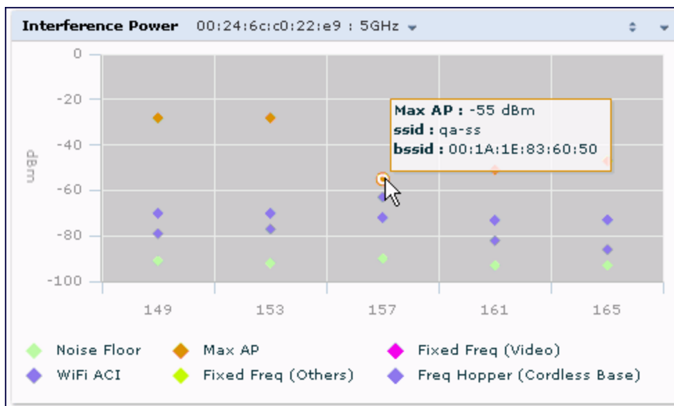
Figure 122 Interference Power
