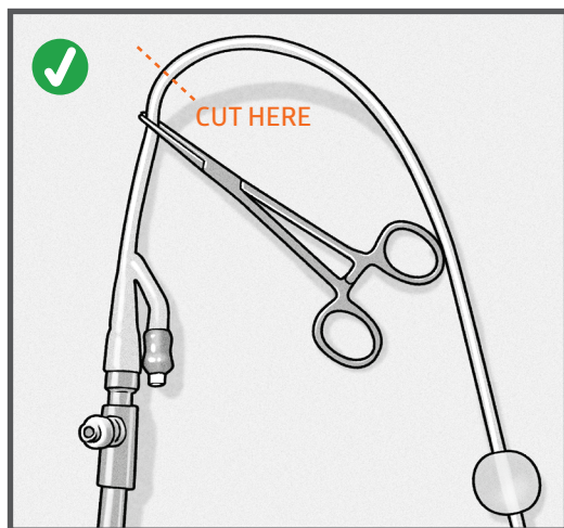
Correct location to cut catheter
