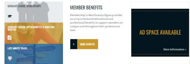
Homepage Square
