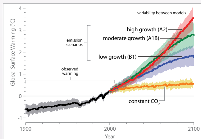
Temperature projections to the year 2100, based on a range of emission scenarios and global climate models. Scenarios that assume the highest growth in greenhouse gas emissions provide the estimates in the top end of the temperature range. The orange line ("constant CO 2 ") projects global temperatures with greenhouse gas concentrations stabilized at year 2000 levels. Source: NASA (adapted from IPCC, 2007)
